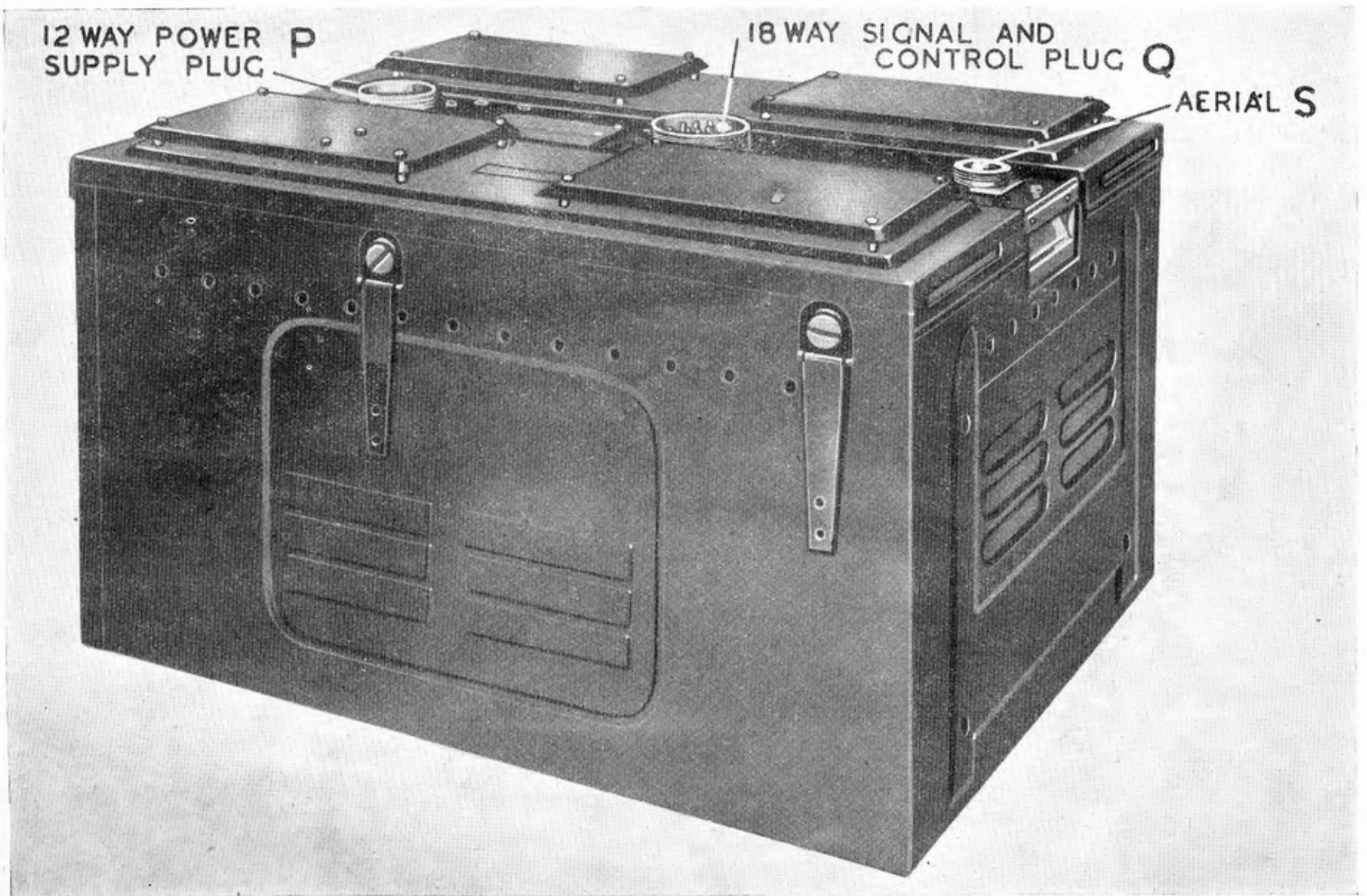
Fig. 1—TR. 1143A—general view.
