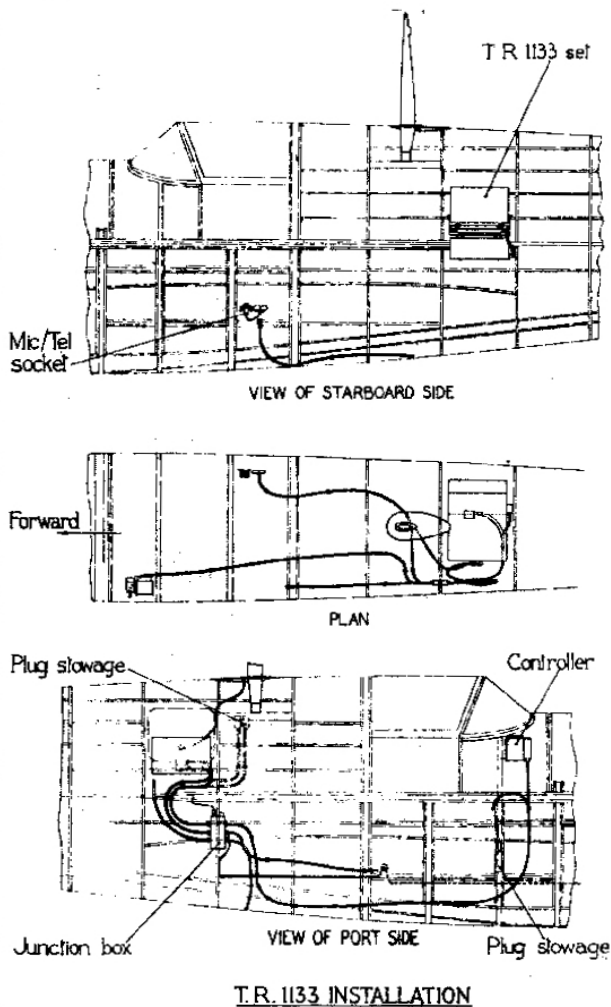
13 (see also 6 & 7): TR1133 installation in the Spitfire Mk. I: this was designed to be interchangeable with the TR9D, as described in the June 1940 Spitfire I pilot's and maintenance manual. The triangular pulley insulator was removed from the head of the mast, leaving the small, scalloped securing bracket at the rear.
