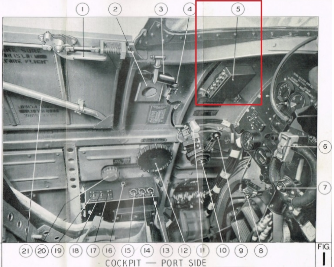
12: Controller Type 3 in the cockpit: although this illustration is from the Pilot's Notes for Spitfire Mk's VII and VIII, the position remained the same from the Spitfire Mk. I, through to the F/FR Mk XIV and P.R. Mk XIX. Post-war, the controller was often mounted horizontally and slightly closer to the instrument panel. [From A.P. 1565 G & H – P.N. Pilot's Notes for Spitfire F.Mk. VII – Merlin 64 or 71 Engine F.MK. VIII – Merlin 63, 66 or 70 Engine: December 1943.]
